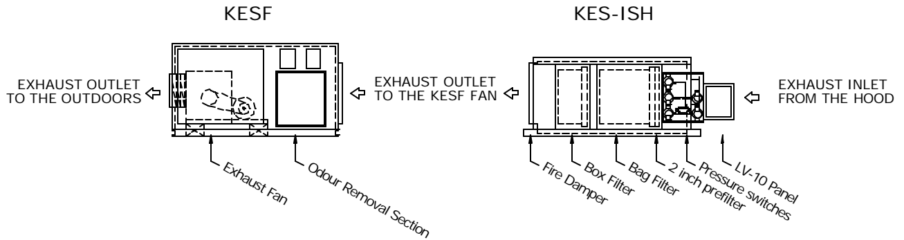
KES-ISH and KESF Enviro components Figure 2
